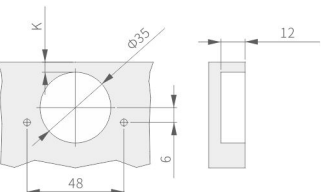
孔距:48mm
