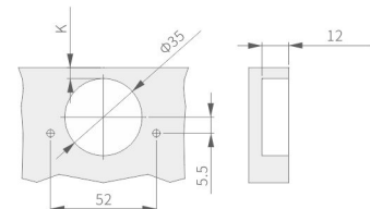
孔距:52mm
