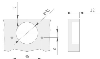
孔距:48mm
