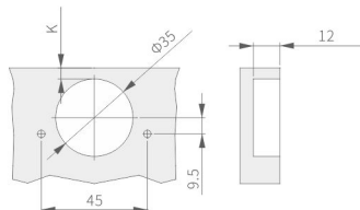
孔距:45mm
