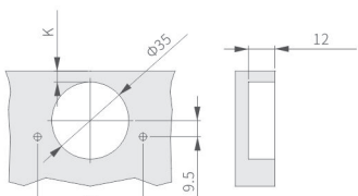
孔距:45mm
