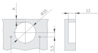
孔距:52mm
