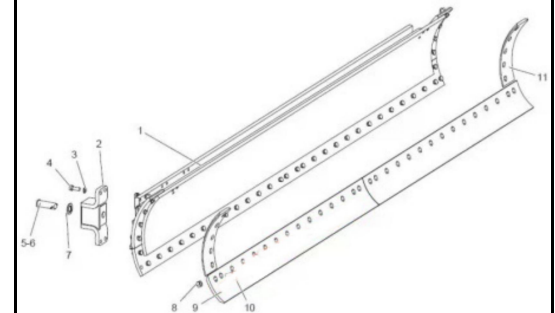
SEM660B Auxiliary blade plate 5332655
