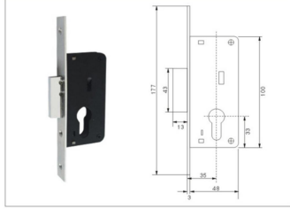
Model:Sliding mortise lock-35mm
