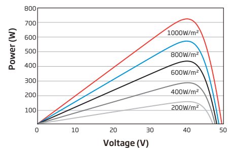
P-V CURVES OF PV MODULE (730W)
