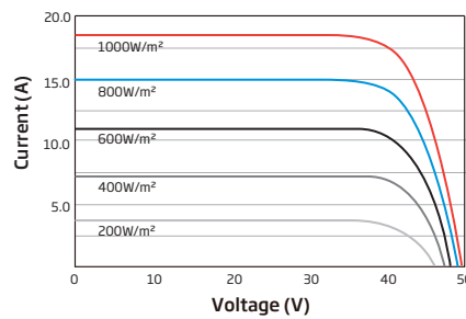
I-V CURVES OF PV MODULE (730W)
