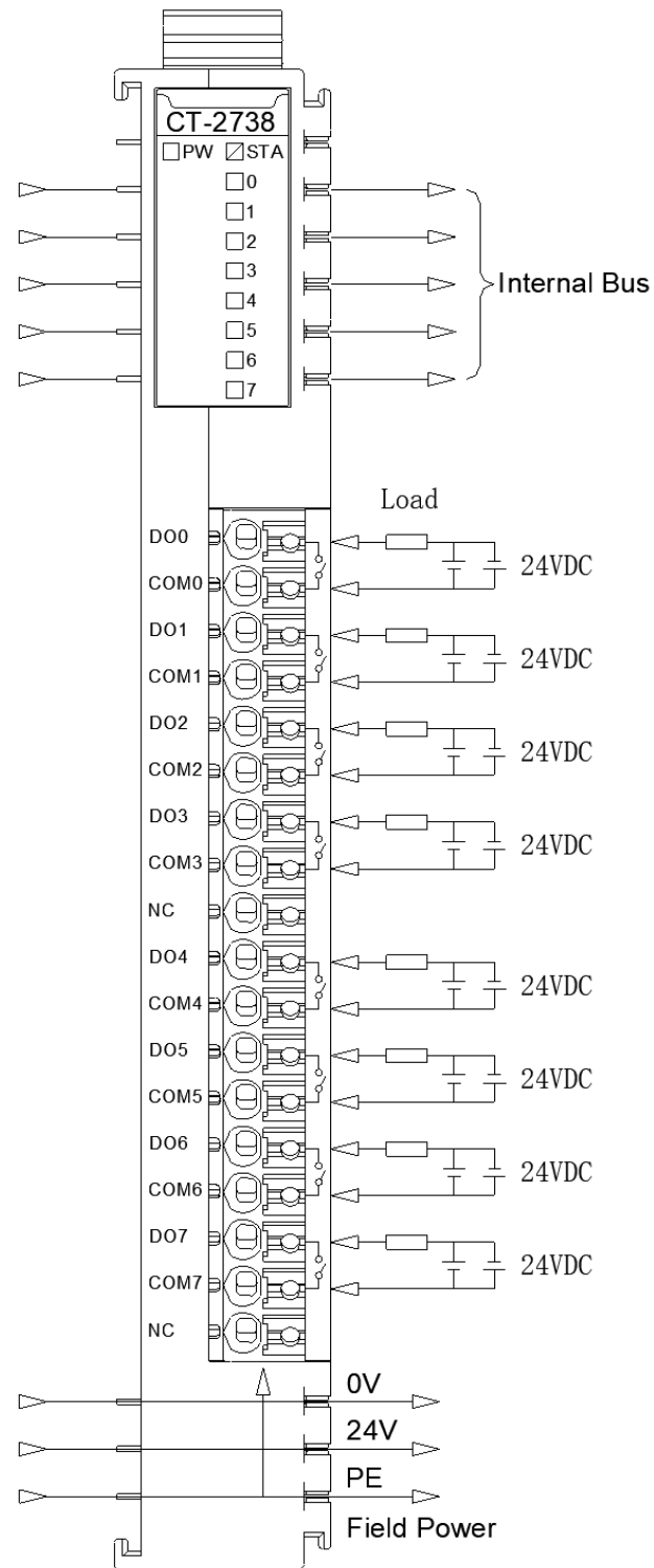
Figure 1 Resistive load wiring diagram
