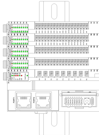
④ Vertical installation
