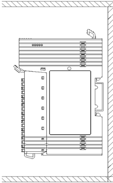
① Right view of horizontal installation
