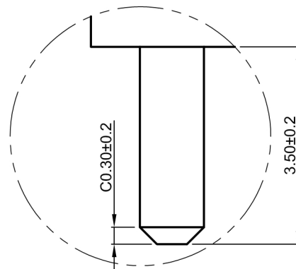
DETAIL B(3:1)
