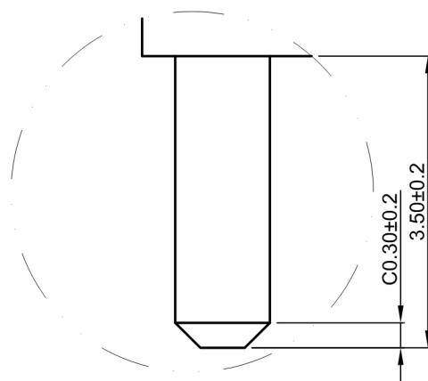
DETAIL B(2:1)
