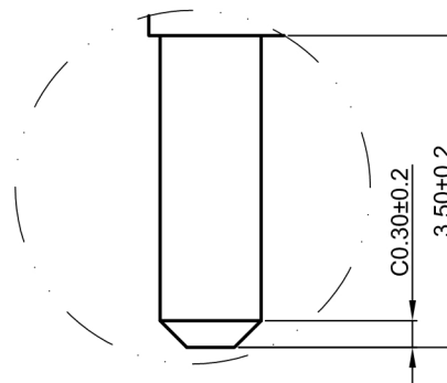
DETAIL B(2:1)
