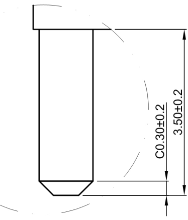
DETAIL B(2:1)
