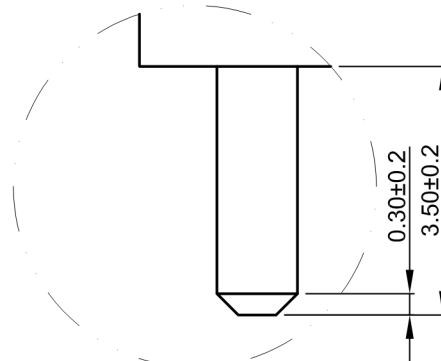
DETAIL B(3:1)
