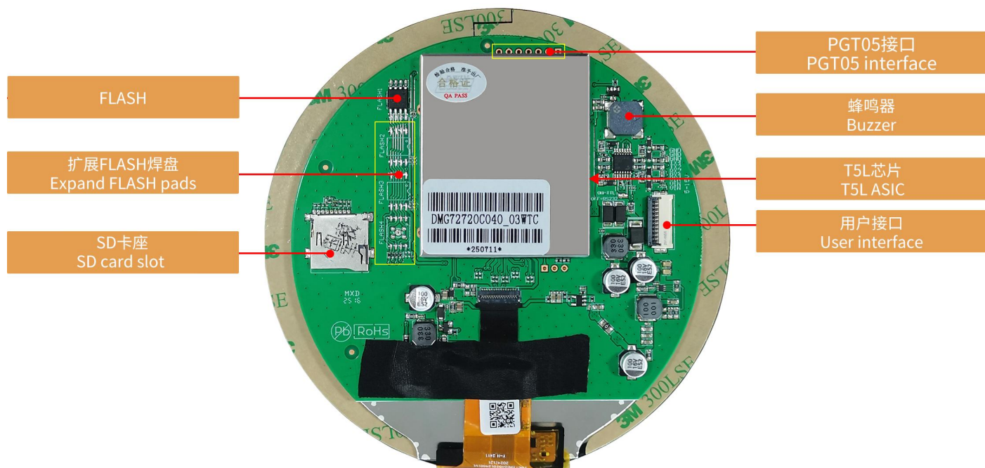
硬件接口图 Hardware interface diagram
