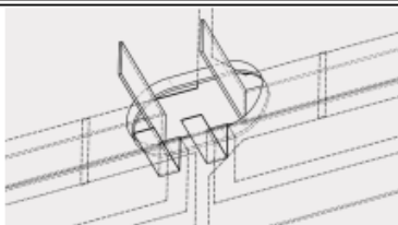
Intermediate junction box welding
