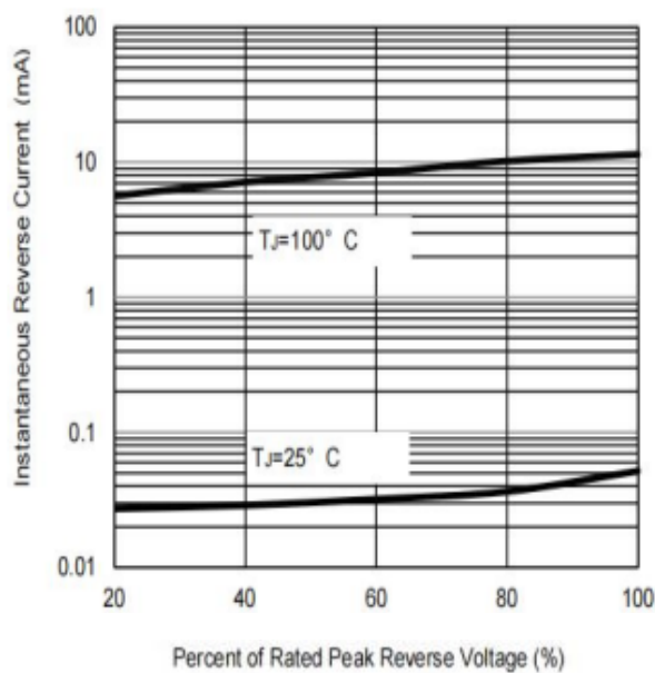
FIG. 3-TYPICAL REVERSE CHARACTERISTICS
