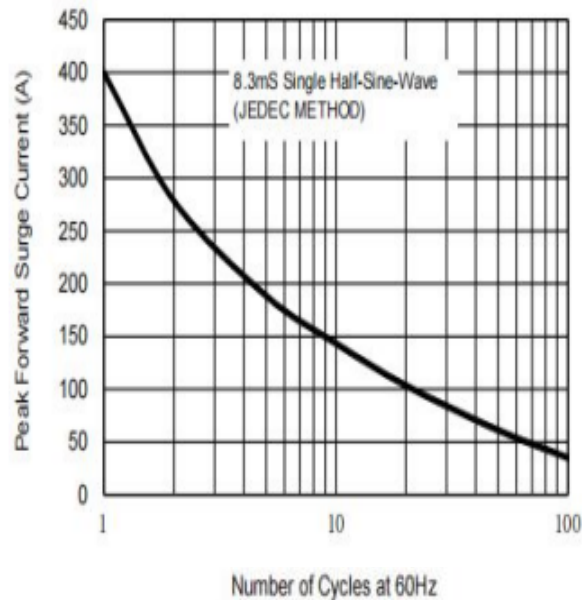
FIG. 2- MAXIMUM NON-REPETITIVE SURGE
