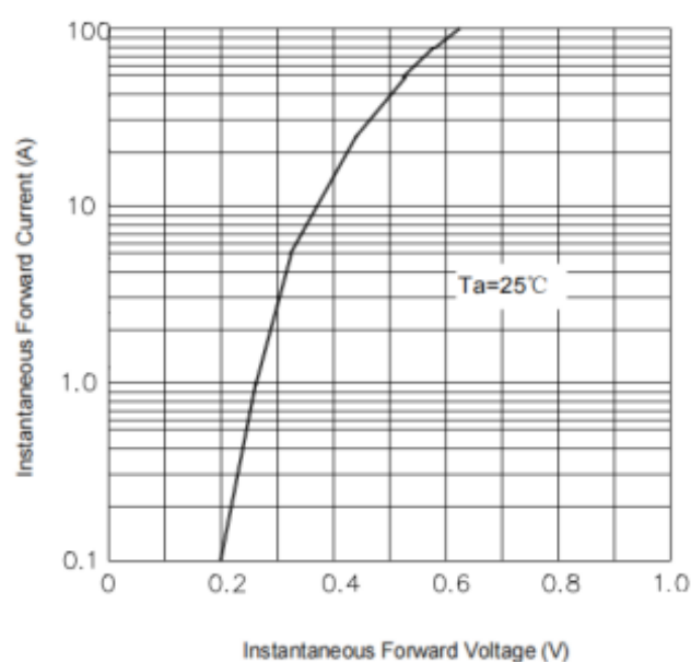
FIG. 4-TYPICAL FORWARD CHARACTERISTICS
