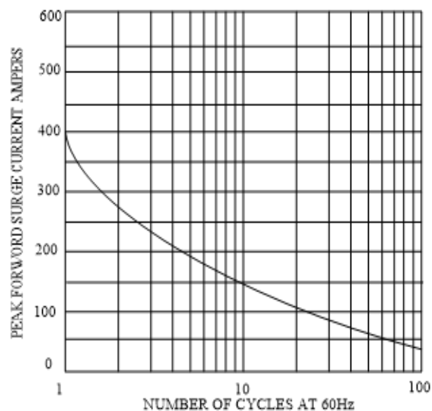
FIG. 2- MAXIMUM NON-REPETITIVE SURGE
