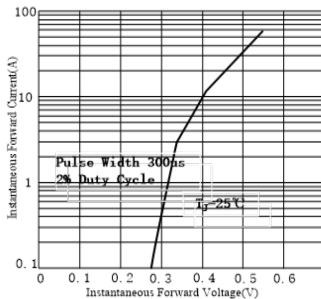
FIG. 4-TYPICAL FORWARD CHARACTERISTICS
