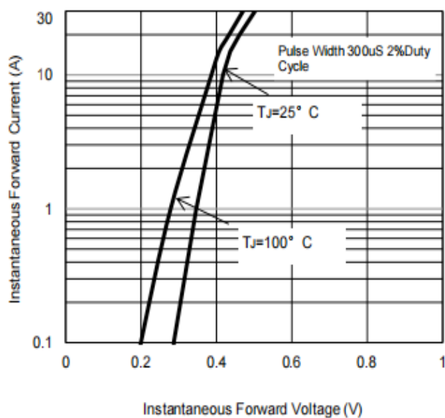
FIG. 4-TYPICAL FORWARD CHARACTERISTICS
