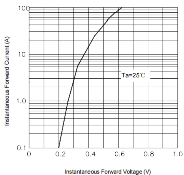
FIG. 4-TYPICAL FORWARD CHARACTERISTICS
