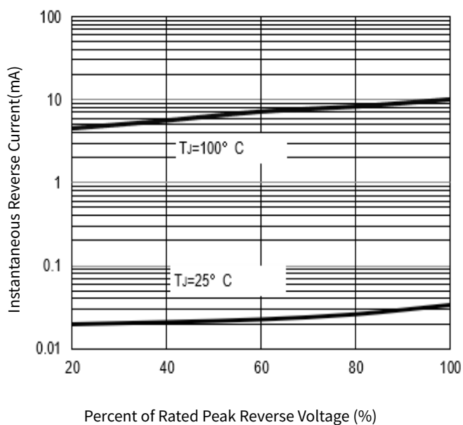
FIG. 3-TYPICAL REVERSE CHARACTERISTICS
