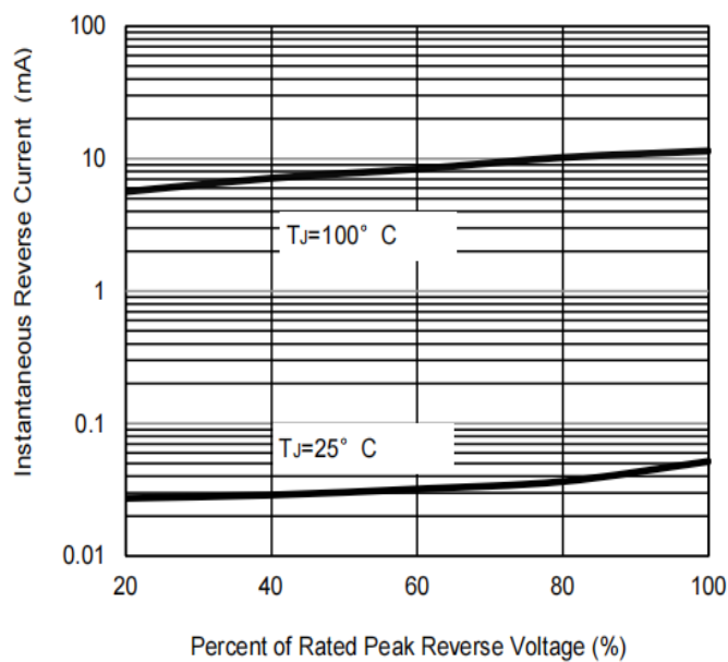
FIG. 3-TYPICAL REVERSE CHARACTERISTICS
