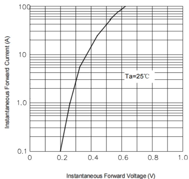
FIG. 4-TYPICAL FORWARD CHARACTERISTICS
