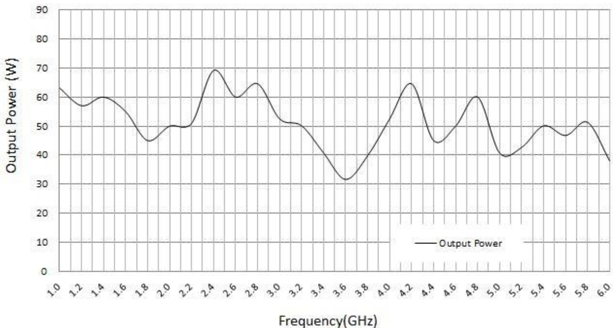
Output Power (Normal temp. +25±3°C)
