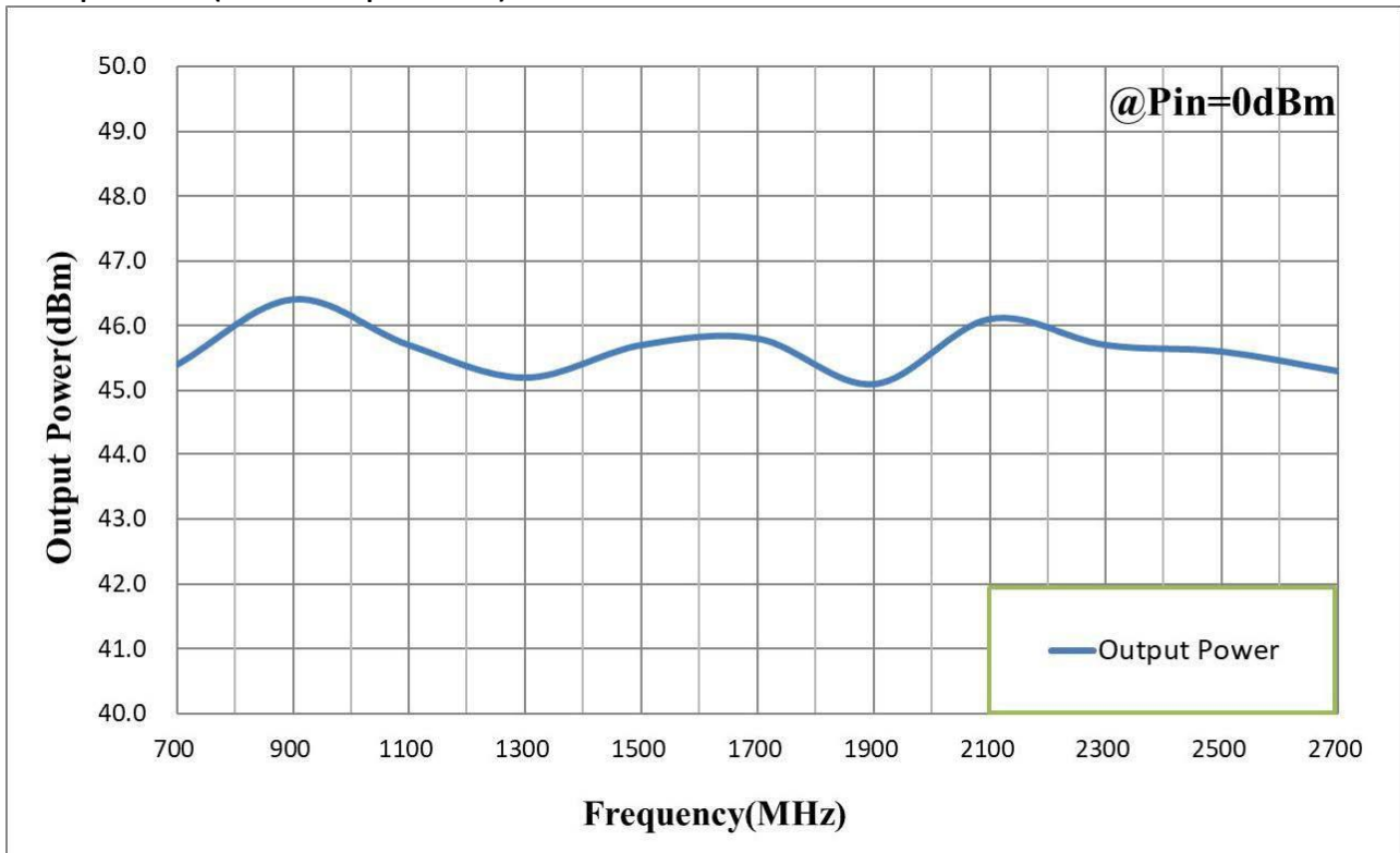
Output Power (Normal temp. +25±3°C)
